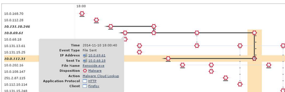
Figure 5. File Trajectory
