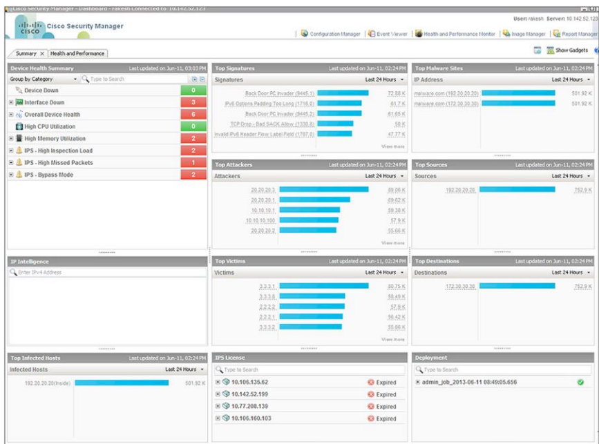
Figure 1. Dashboard
